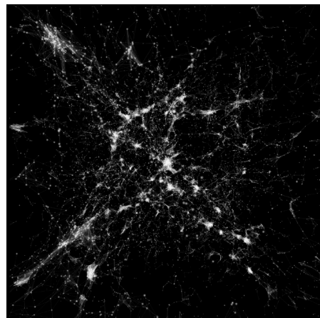
Formation of a galaxy cluster at a node of the cosmic web
